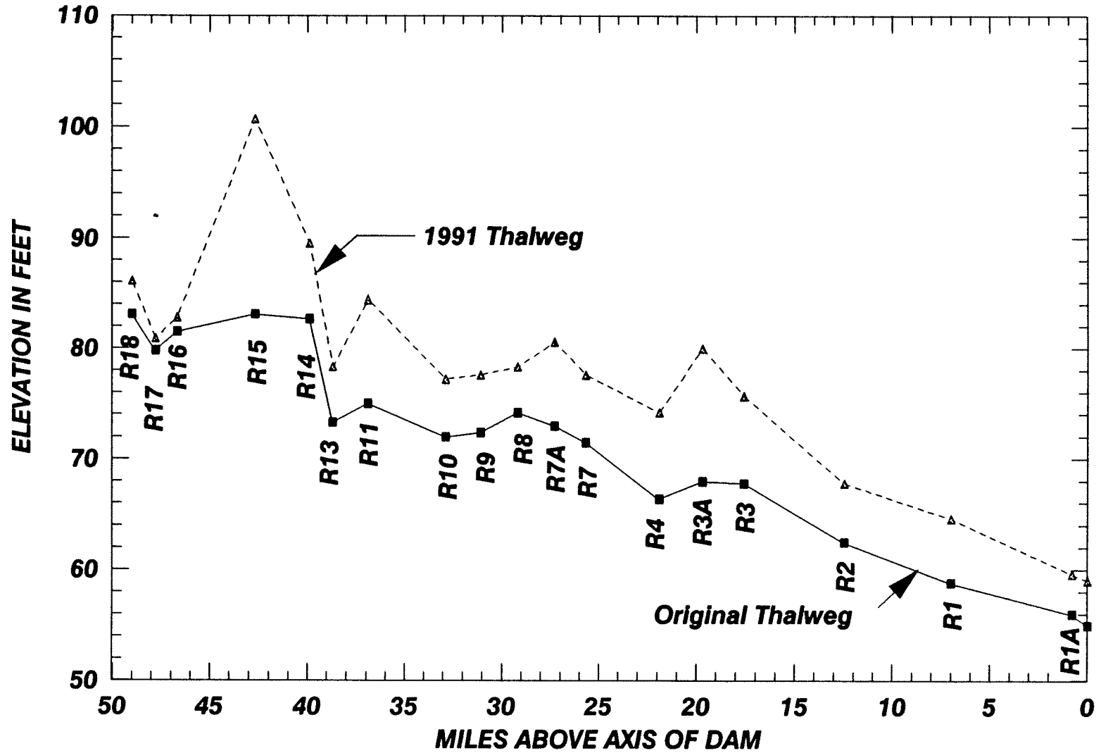
Figure 4. – Longitudinal profile – Trinity River.
